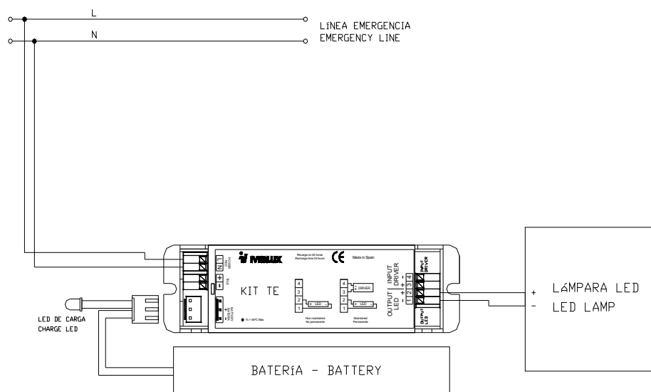
ESQUEMA CONEXIONADO KIT EMERGENCIA LED TE WIRING DIAGRAM TE LED EMERGENCY KIT
