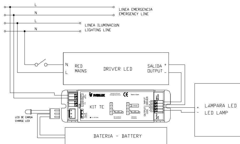
ESQUEMA CONEXIONADO KIT PERMANENTE LED TE WIRING DIAGRAM TE LED MANTAINED KIT
