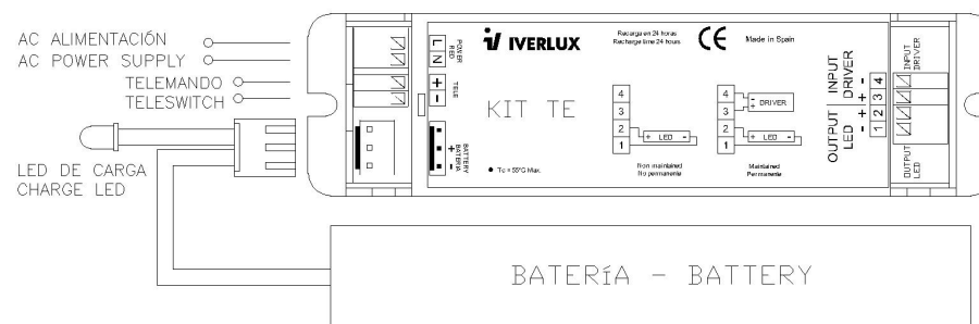
ESQUEMA CONEXIONADO KIT EMERGENCIA LED TE WIRING DIAGRAM TE LED EMERGENCY KIT
